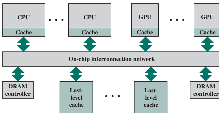
Figure 18.7 Heterogeneous Multicore Chip Elements
