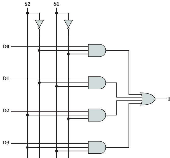
Figure 11.13 Multiplexer Implementation
