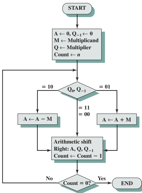
Figure 10.12 Booth's Algorithm for Two's Complement Multiplication
