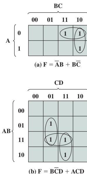
Figure 11.9 Overlapping Groups
