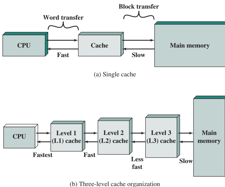
Figure 4.3 Cache and Main Memory
