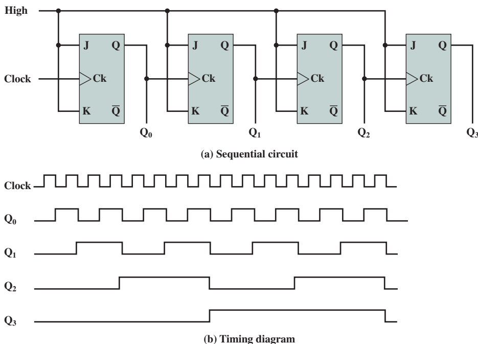
Figure 11.30 Ripple Counter
