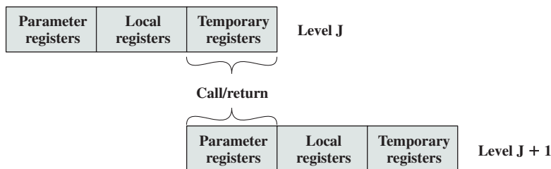
Figure 15.1 Overlapping Register Windows
