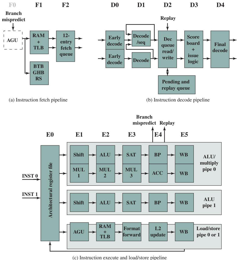
Figure 16.10 ARM Cortex-A8 Integer Pipeline
