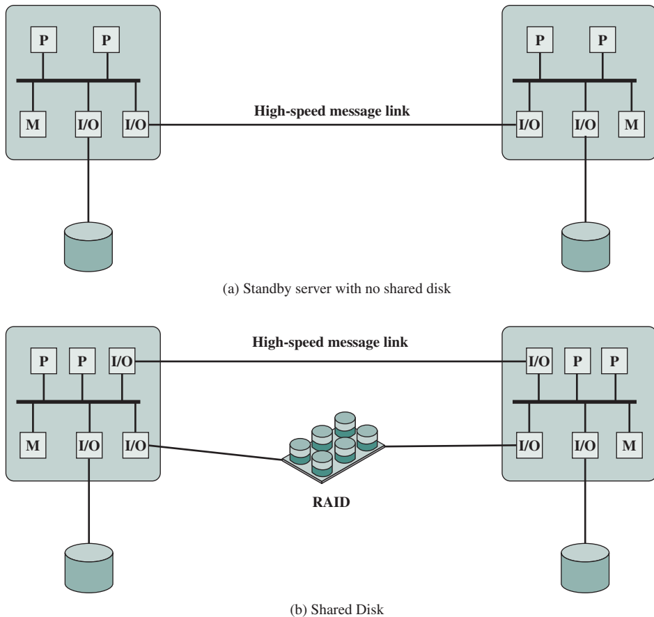
Figure 17.8 Cluster Configurations
